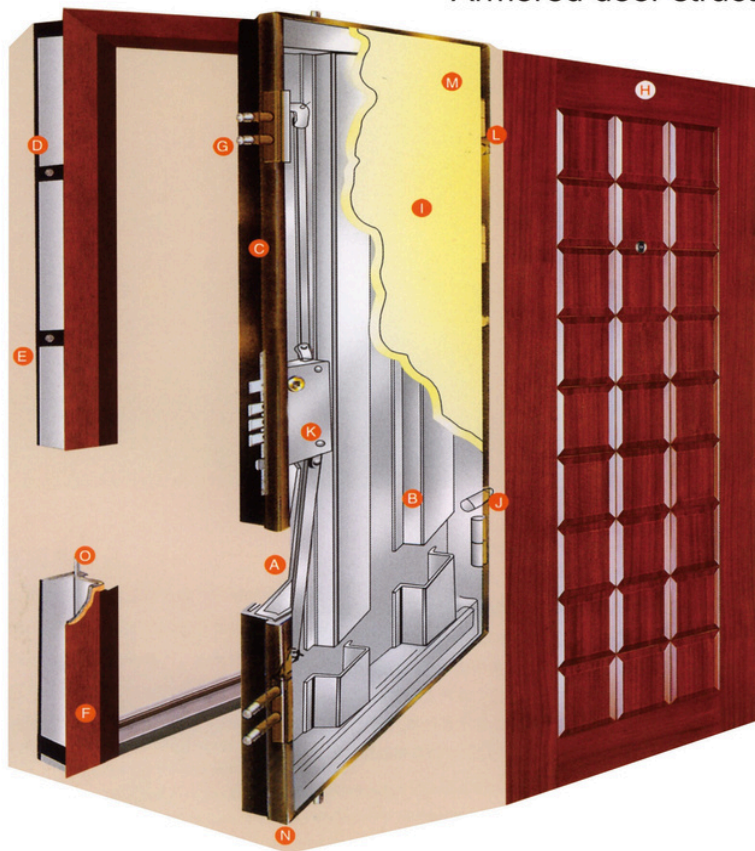
Armored door structure
