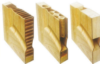
Hollow core/ semiwood/particleboard
